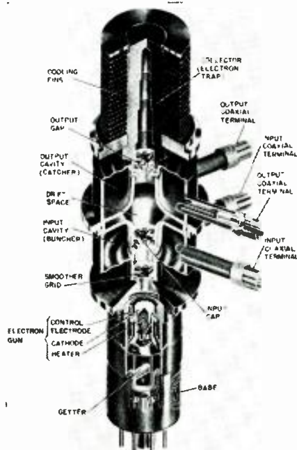
Courtesy Sperry Gyroscope Co. Fig. 5—Cutaway of a typical Klystron tube.
