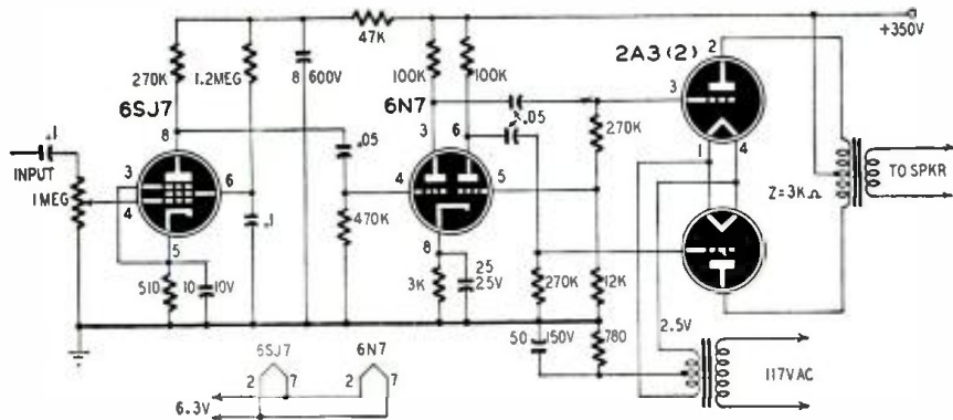
Fig. 5—This simple push-pull amplifier circuit shows how the design information is used.
