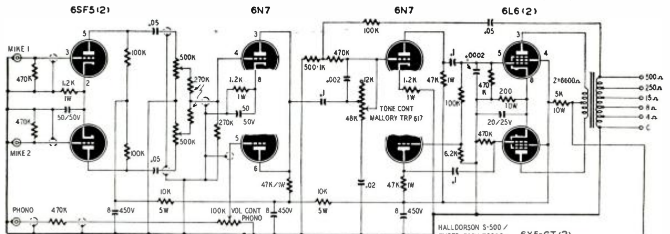
Fig. 1—C4 is .006 µf from 6X5 plate to ground.
