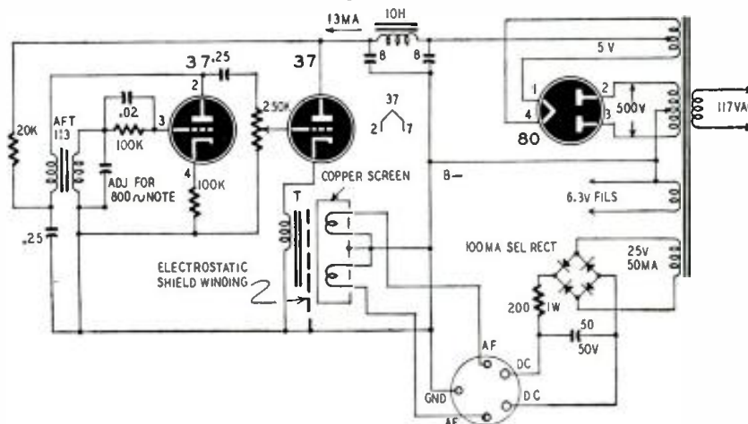
Fig. 3—The tone generator. Note how the output is balanced to avoid upsetting the bridge.
