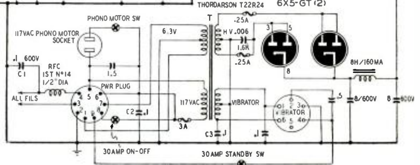
Fig. 1—C4 is .006 µf from 6X5 plate to ground.
