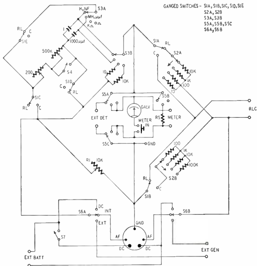
Fig. 2—Switches and controls in the bridge circuit provide for four ranges of R, C, and L.
